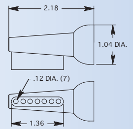
1/2" SIDE-SPRAY NOZZLE
