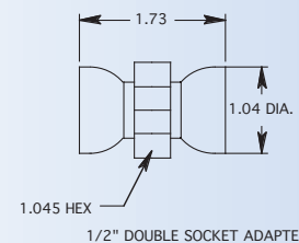
1/2" DOUBLE SOCKET ADAPTER
