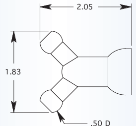
1/2" X 1/4" REDUCER Y - MOLDED STYLE
