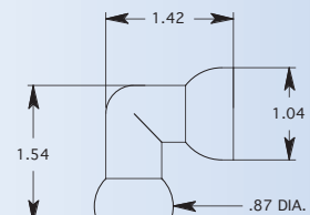
1/2" 90 DEGREE ELBOW
