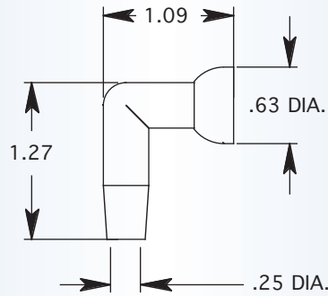
1/4" 90 DEGREE NOZZLE
