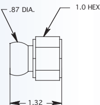
3/8" FPT FEMALE CONNECTOR 1/2" FPT FEMALE CONNECTOR
