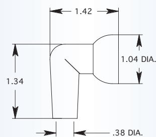
3/8" 90 DEGREE NOZZLE
